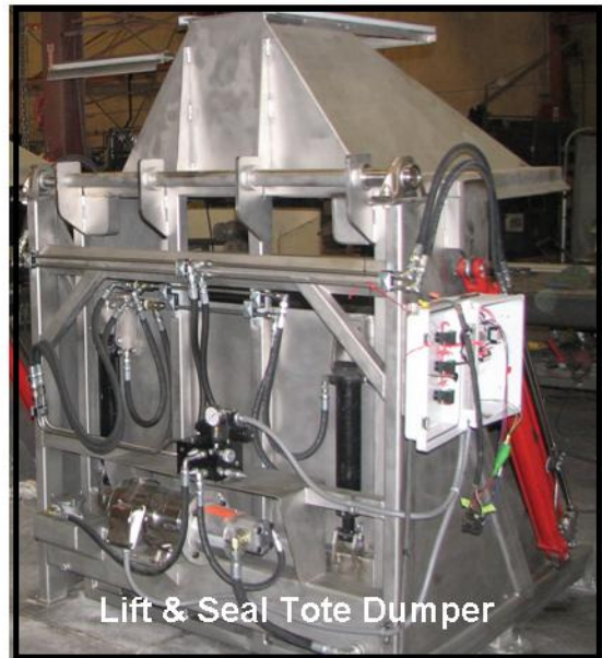
Roll Back Tote Dumper
